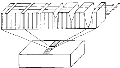
Figure 5.1. Depth setting standard (type A2) with enlarged area of measurement
